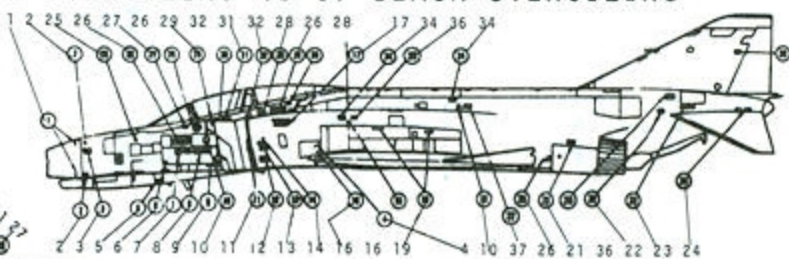
FUSELAGE LEFT SIDE
