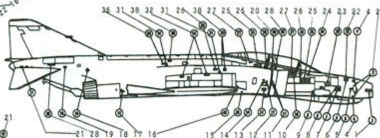
FUSELAGE RIGHT SIDE
